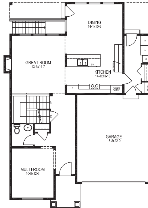
MAIN Approx. 1100 Sq.Ft.
