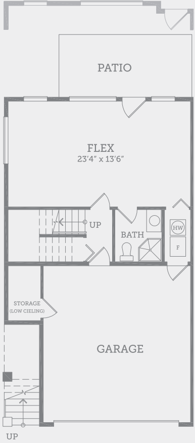
GROUND FLOOR 556 SQ.FT.
